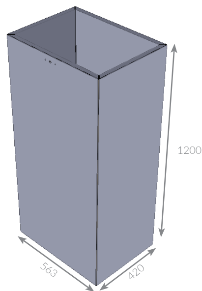
Dreamoc HD3.2 Stand - measurements
