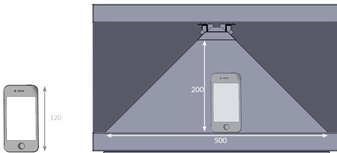
Dreamoc HD3.2 front - object reference
