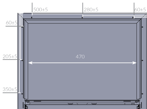
screw measurements
