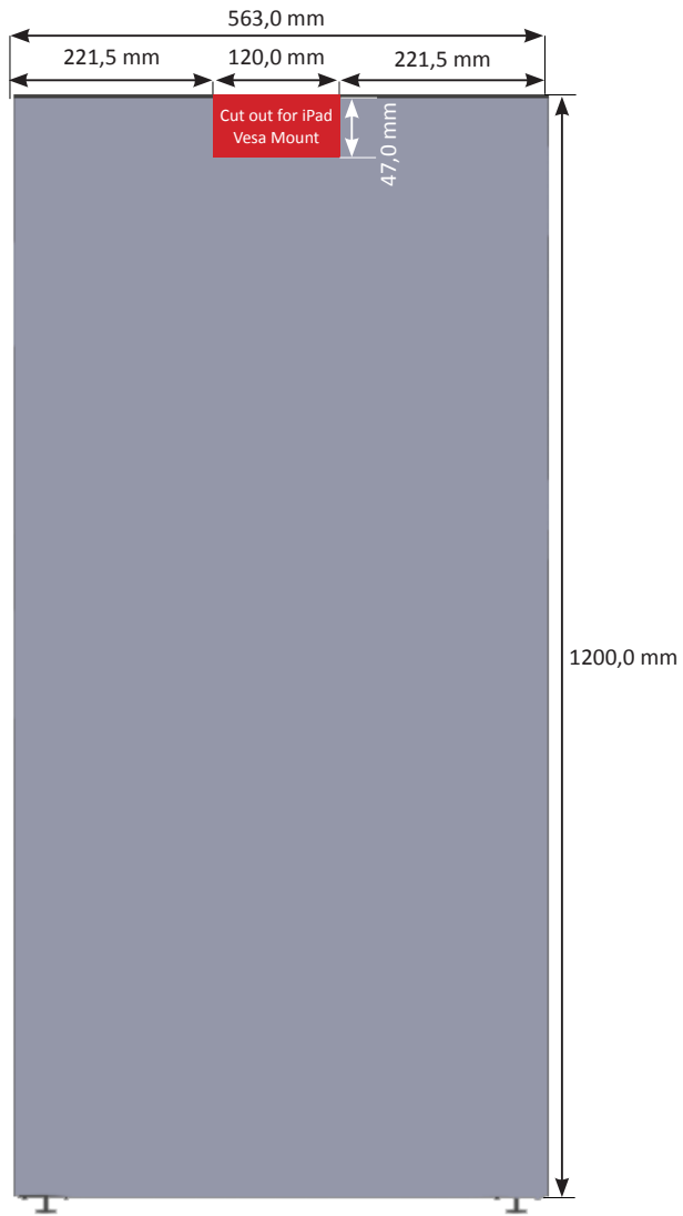
DREAMOC HD3 STAND FRONT VIEW with cut out for iPad Vesa Mount
